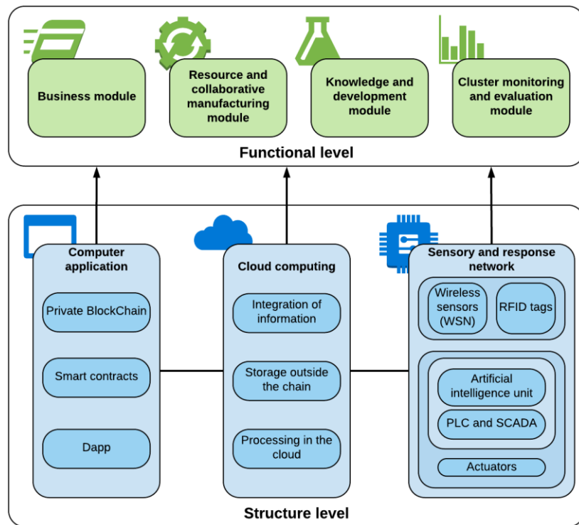
Fig. 4. Architecture of structural and functional levels (The authors)
